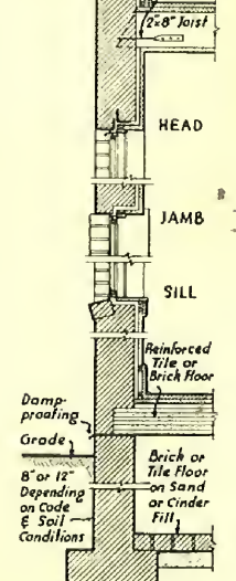
Wall Section
